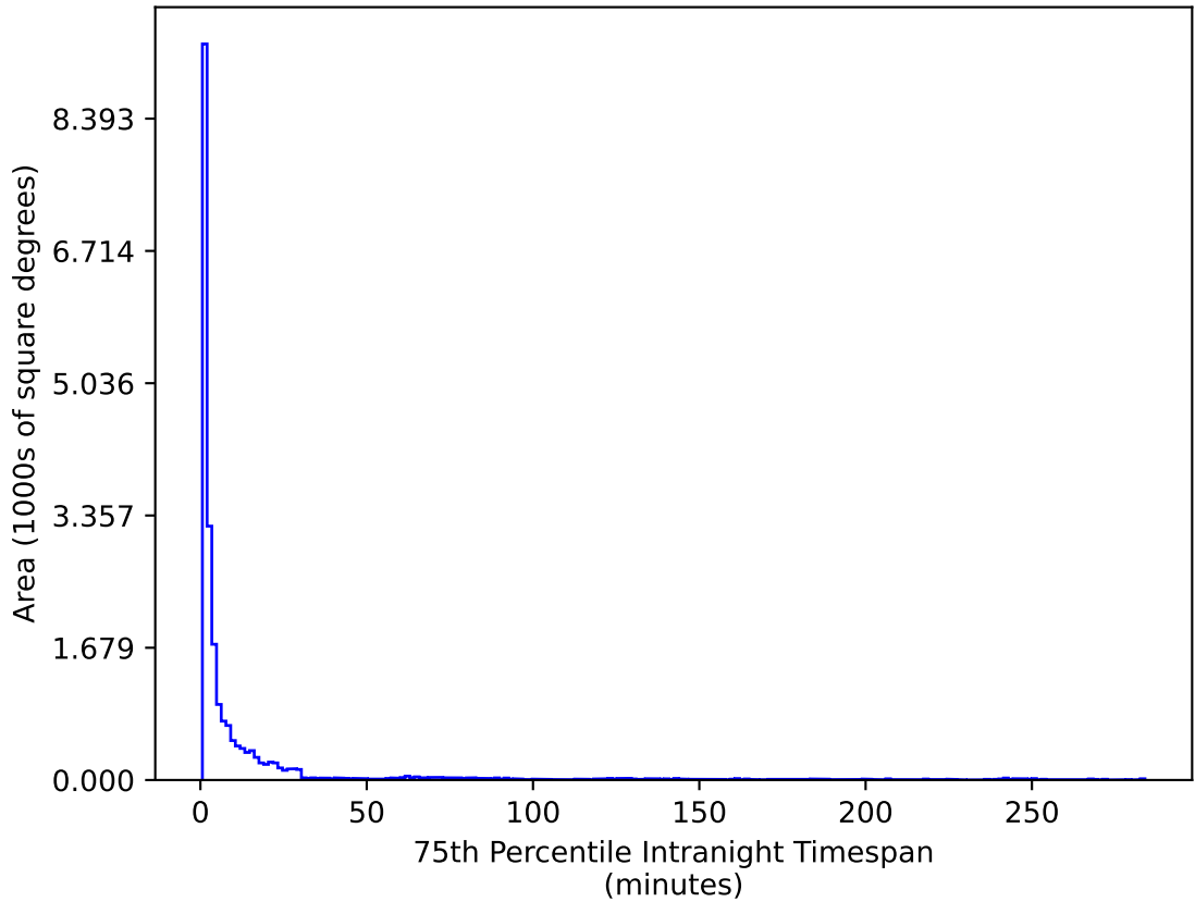
ddf_acor_sf10_lsf15_lsr50_v3.4_10yrs All sky u band: 75th Percentile Intranight Timespan
