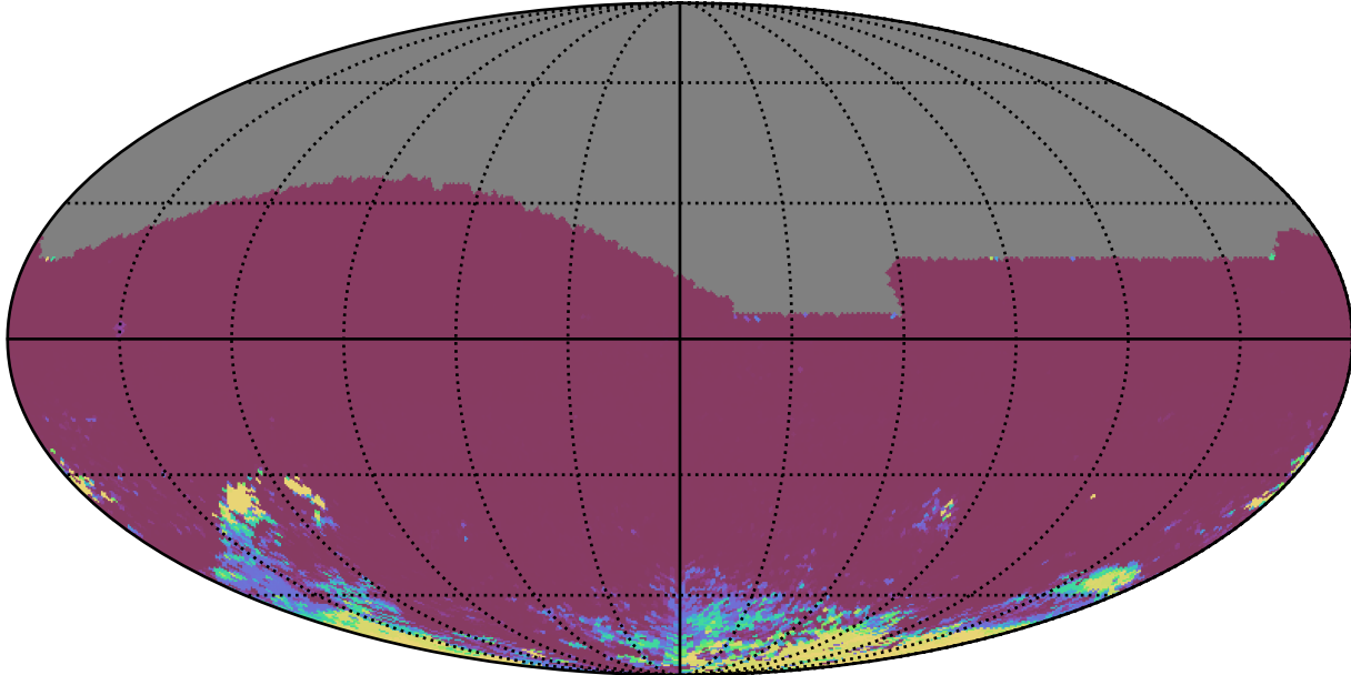
ddf_acor_sf10_lsf15_lsr50_v3.4_10yrs All sky ri bands: 75th Percentile Intranight Timespan
