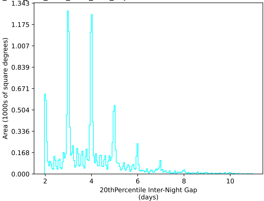
ddf_acor_sf10_ls15_lsr50_v3.4_10yrs WFD u band: 20thPercentile Inter-Night Gap
