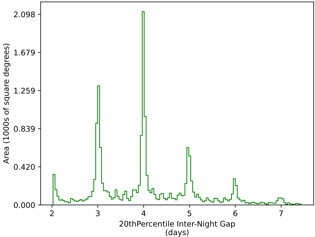
ddf_acor_sf10_ls15_lsr50_v3.4_10yrs WFD g band: 20thPercentile Inter-Night Gap
