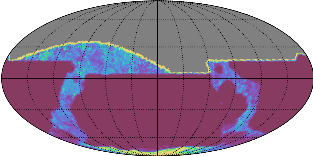
ddf_acor_sf10_lsf15_lsr50_v3.4_10yrs All sky all bands: 20thPercentile Inter-Night Gap
