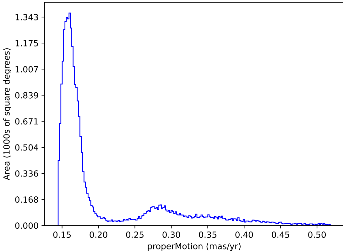
ddf_acor_sf10_ls15_lsr50_v3.4_10yrs : properMotion
