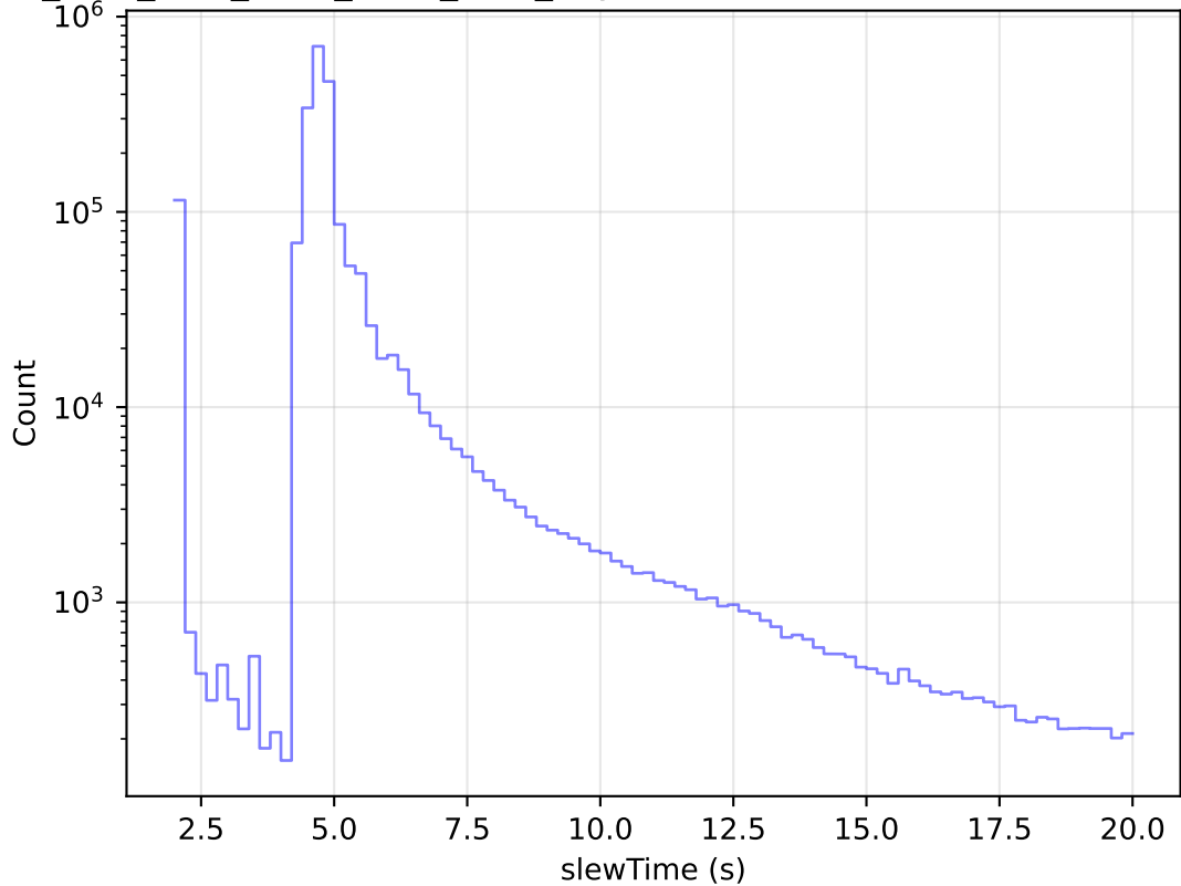
ddf_acor_sf10_Isf15_Isr50_v3.4_10yrs All visits: Zoom Slew Time Histogram
