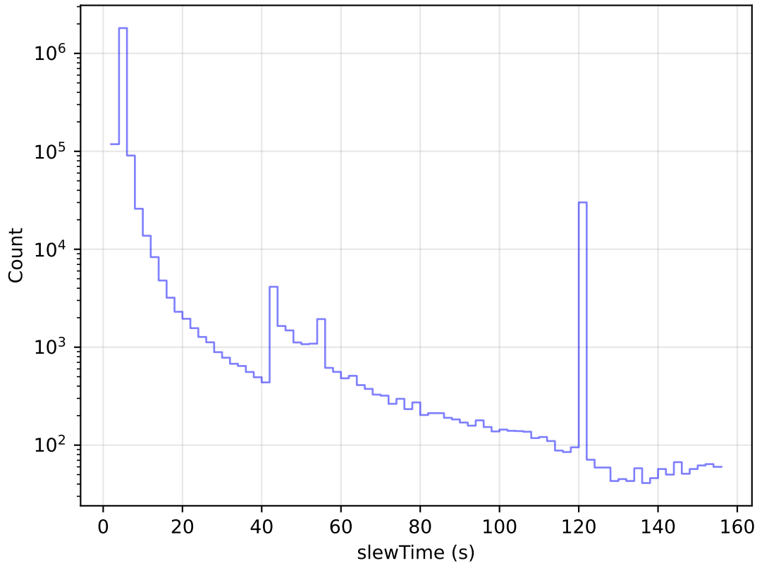
ddf_acor_sf10_lsf15_lsr50_v3.4_10yrs All visits: Slew Time Histogram
