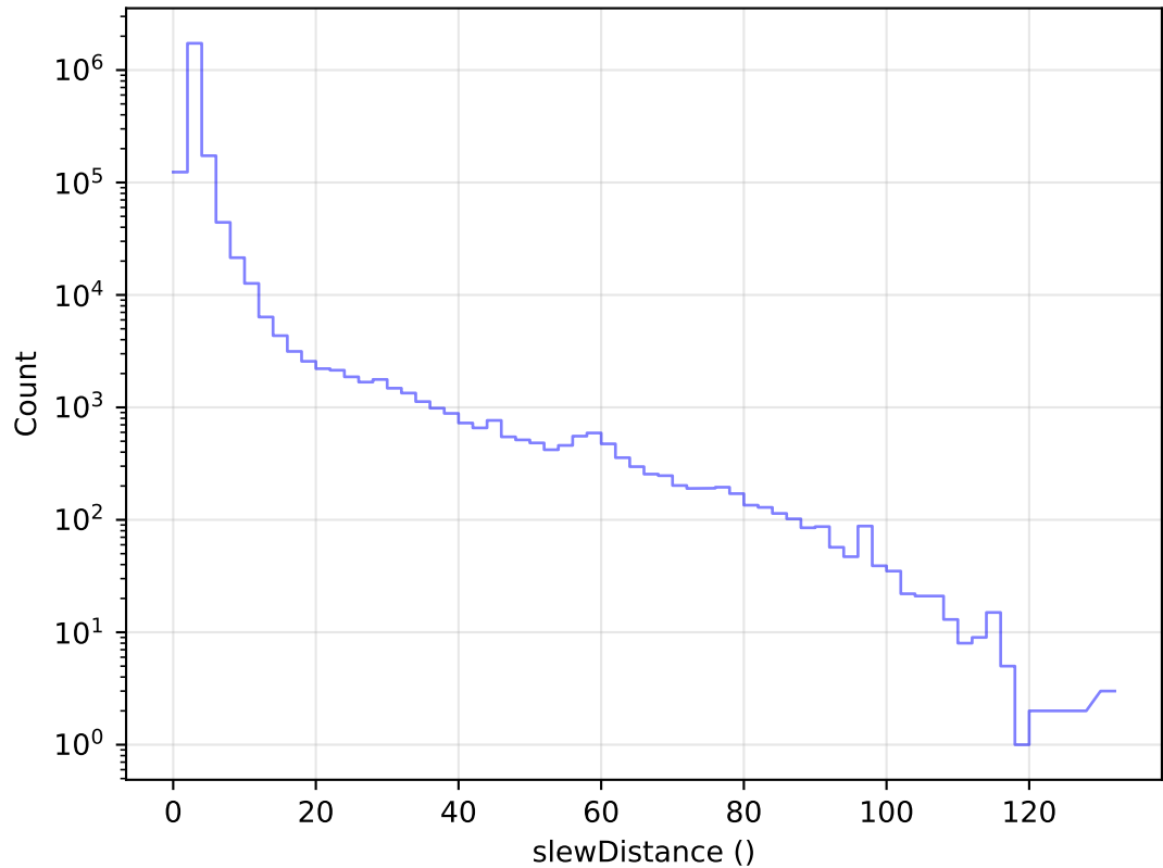
ddf_acor_sf10_lsf15_lsr50_v3.4_10yrs All visits: Slew Distance Histogram
