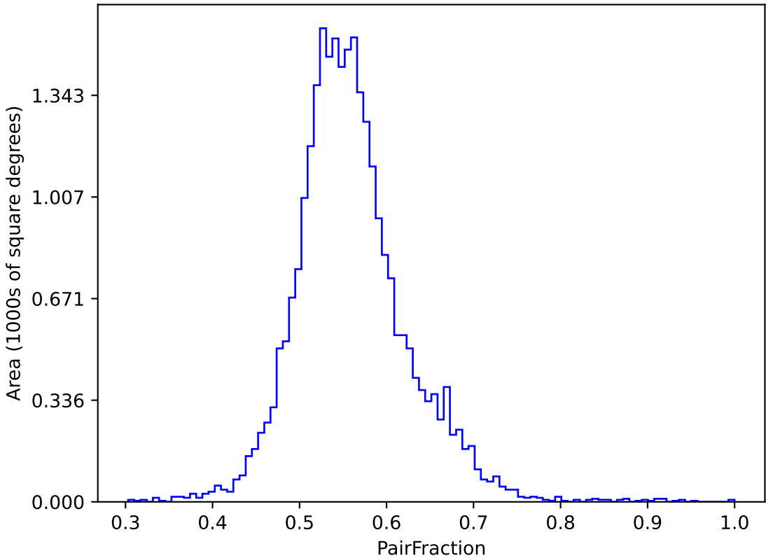
ddf_acor_sf10_lsf15_lsr50_v3.4_10yrs (g or r or i): PairFraction
