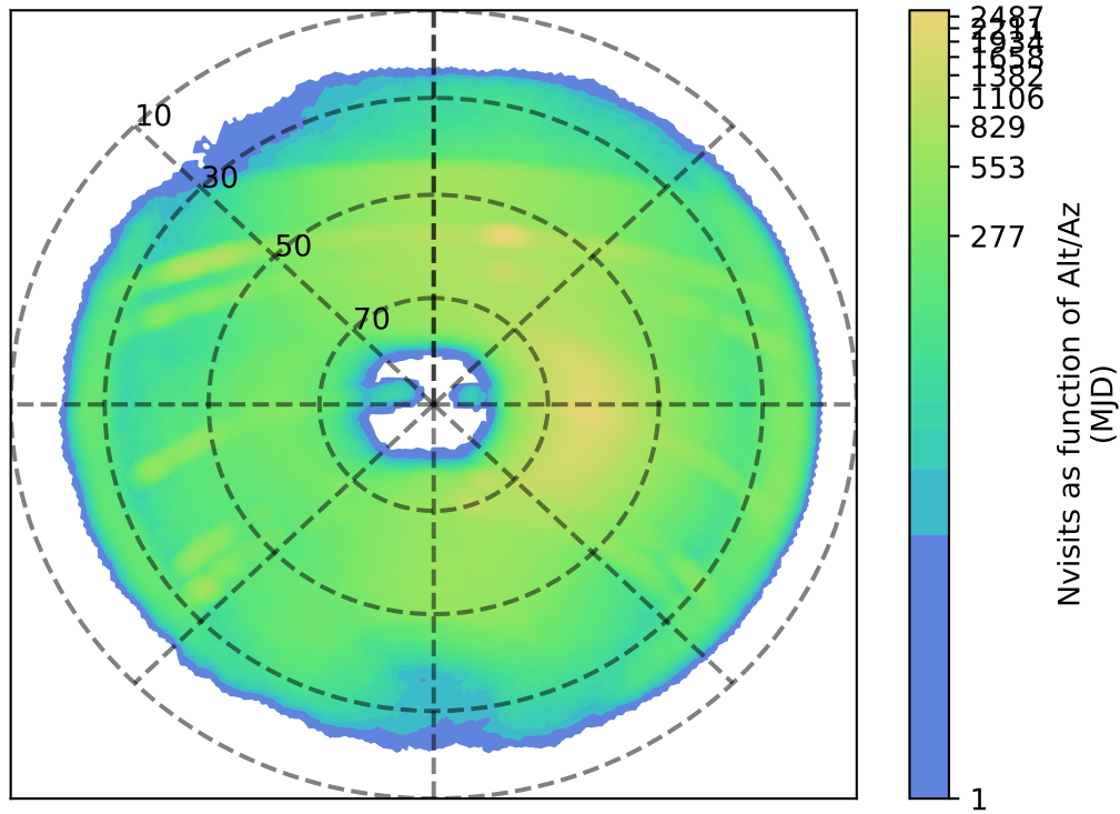
ddf_acor_sf10_ls15_lsr50_v3.4_10yrs z: Nvisits as function of Alt/Az
