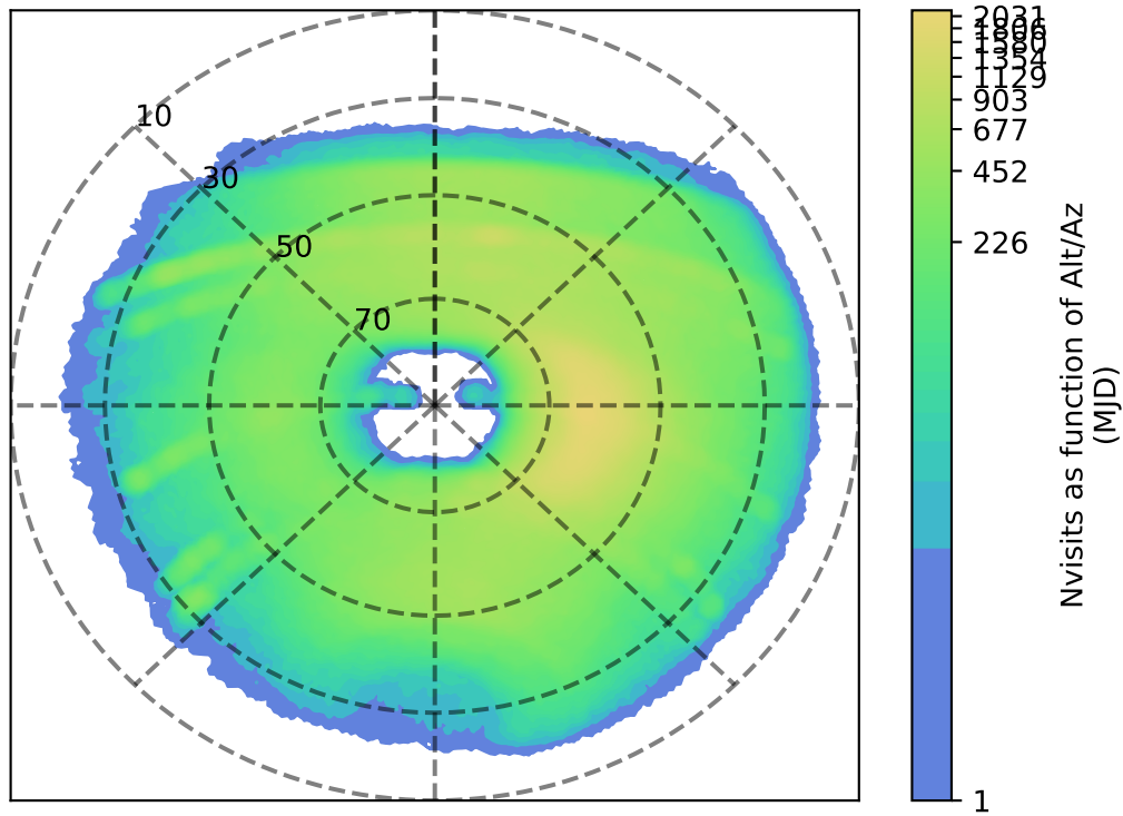
ddf_acor_sf10_lsf15_lsr50_v3.4_10yrs y: Nvisits as function of Alt/Az
