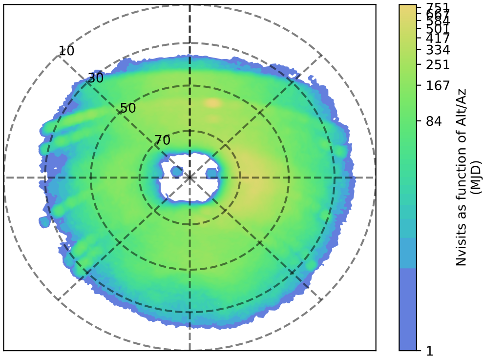
ddf_acor_sf10_ls15_lsr50_v3.4_10yrs u: Nvisits as function of Alt/Az
