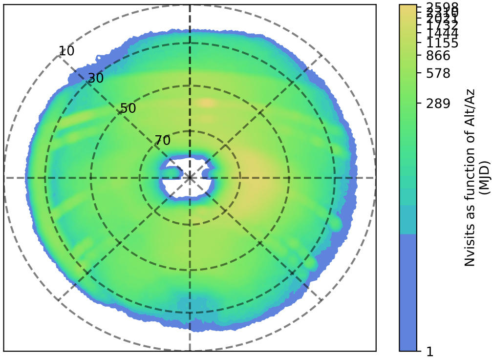
ddf_acor_sf10_ls15_lsr50_v3.4_10yrs r: Nvisits as function of Alt/Az
