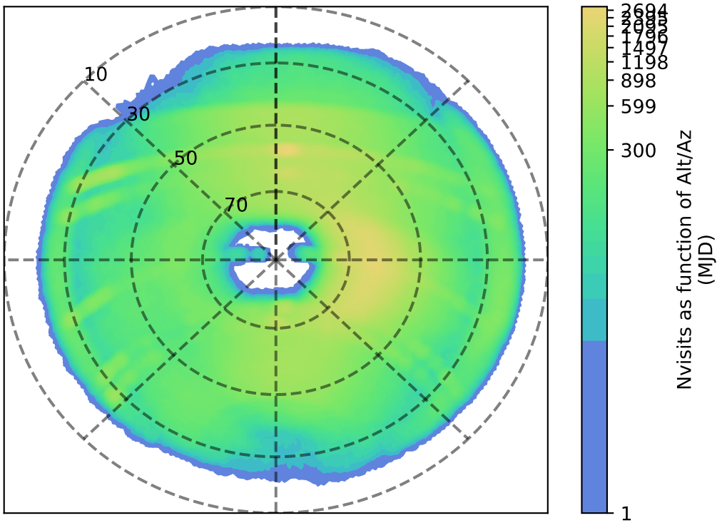
ddf_acor_sf10_ls15_lsr50_v3.4_10yrs i: Nvisits as function of Alt/Az
