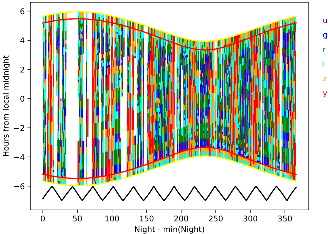
ddf_acor_sf10_lsf15_lsr50_v3.4_10yrs year 8-9: Hourglass
