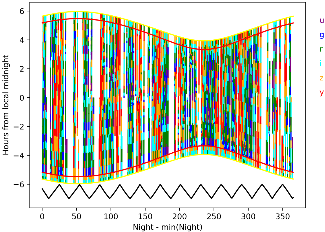
ddf_acor_sf10_lsf15_lsr50_v3.4_10yrs year 7-8: Hourglass
