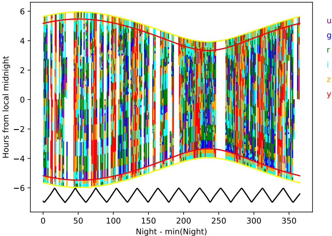
ddf_acor_sf10_lsf15_lsr50_v3.4_10yrs year 5-6: Hourglass
