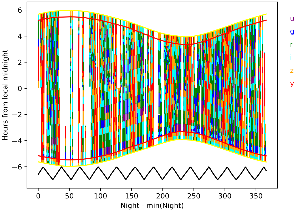
ddf_acor_sf10_lsf15_lsr50_v3.4_10yrs year 3-4: Hourglass
