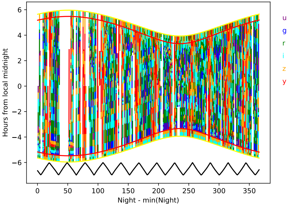
ddf_acor_sf10_lsf15_lsr50_v3.4_10yrs year 2-3: Hourglass
