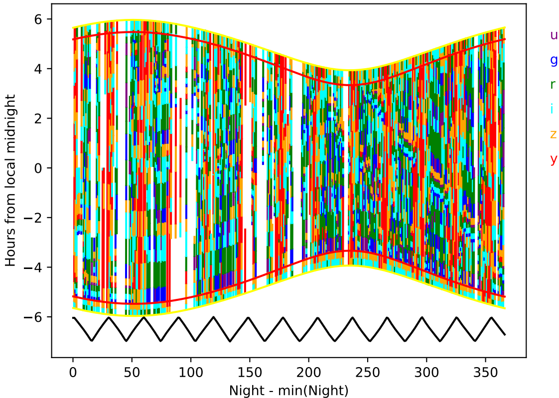
ddf_acor_sf10_lsf15_lsr50_v3.4_10yrs year 1-2: Hourglass
