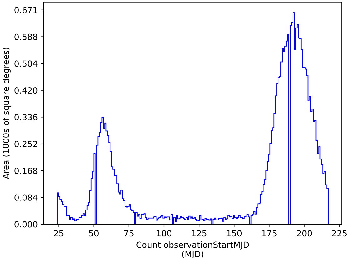
ddf_acor_sf10_lsf15_lsr50_v3.4_10yrs i: Count observationStartMJD
