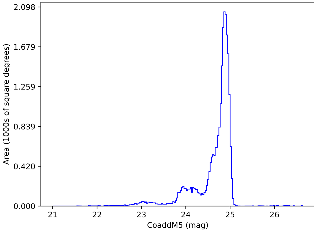
ddf_acor_sf10_lsf15_lsr50_v3.4_10yrs y: CoaddM5
