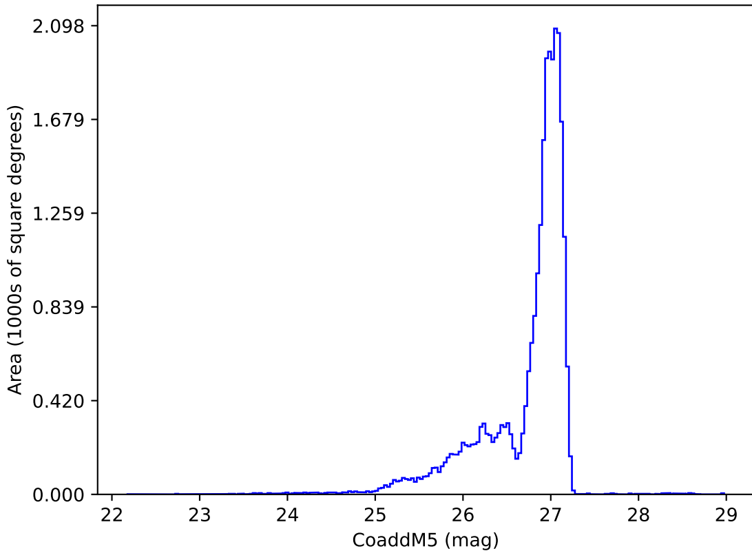
ddf_acor_sf10_lsf15_lsr50_v3.4_10yrs r: CoaddM5
