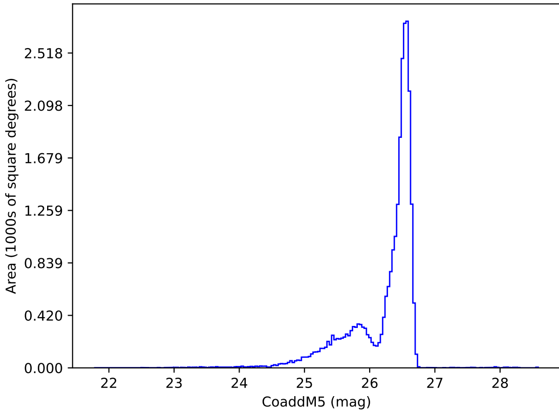
ddf_acor_sf10_ls15_lsr50_v3.4_10yrs i: CoaddM5
