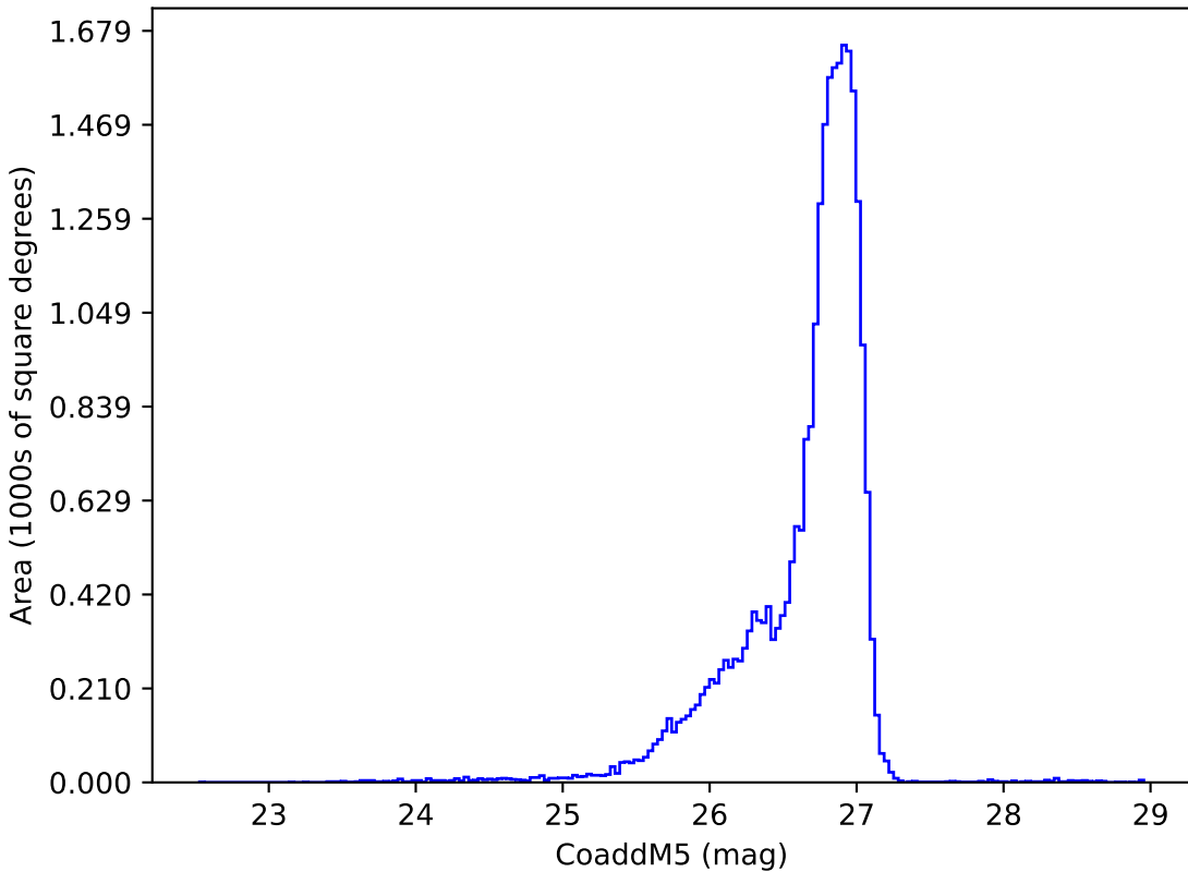
ddf_acor_sf10_lsf15_lsr50_v3.4_10yrs g: CoaddM5
