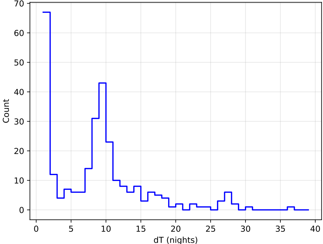
ddf_acor_sf10_Isf15_Isr50_v3.4_10yrs all bands: DD:XMM_LSS Delta Nights Histogram
