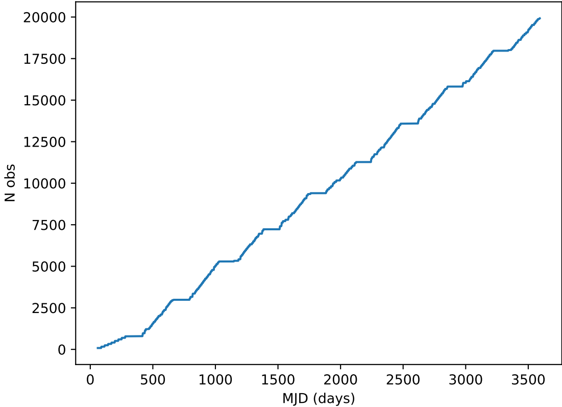
ddf_acor_sf10_lsf15_lsr50_v3.4_10yrs all bands: DD:XMM_LSS Cumulative NVisits
