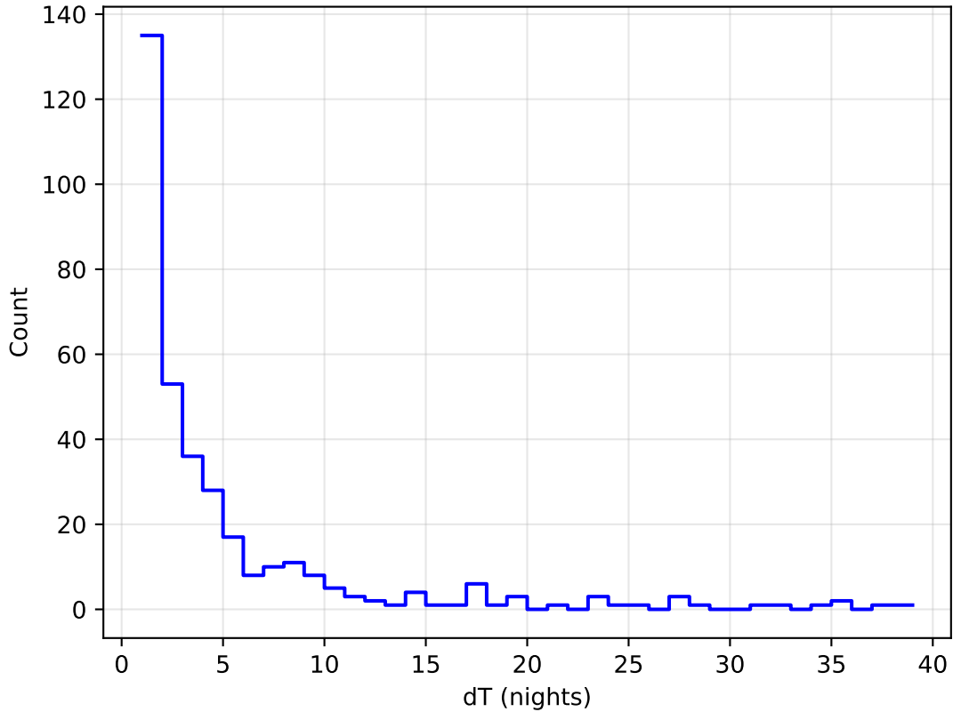
ddf_acor_sf10_lsf15_lsr50_v3.4_10yrs all bands: DD:WFD Delta Nights Histogram
