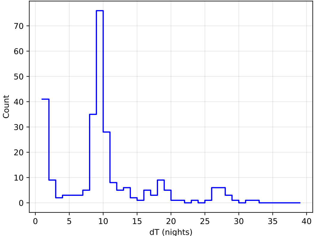
ddf_acor_sf10_lsf15_lsr50_v3.4_10yrs all bands: DD:ELAISS1 Delta Nights Histogram
