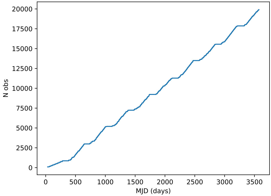
ddf_acor_sf10_lsf15_lsr50_v3.4_10yrs all bands: DD:ELAISS1 Cumulative NVisits
