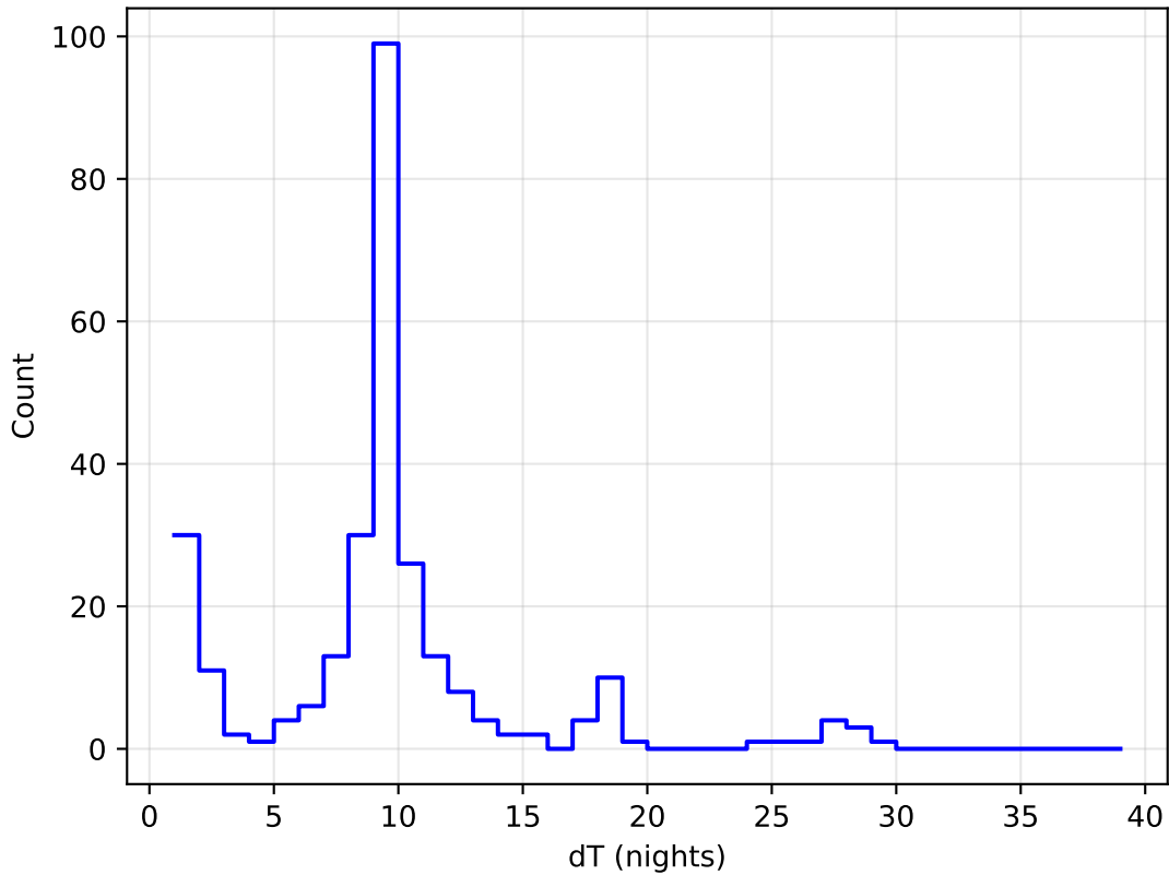
ddf_acor_sf10_ls15_lsr50_v3.4_10yrs all bands: DD:EDFS Delta Nights Histogram
