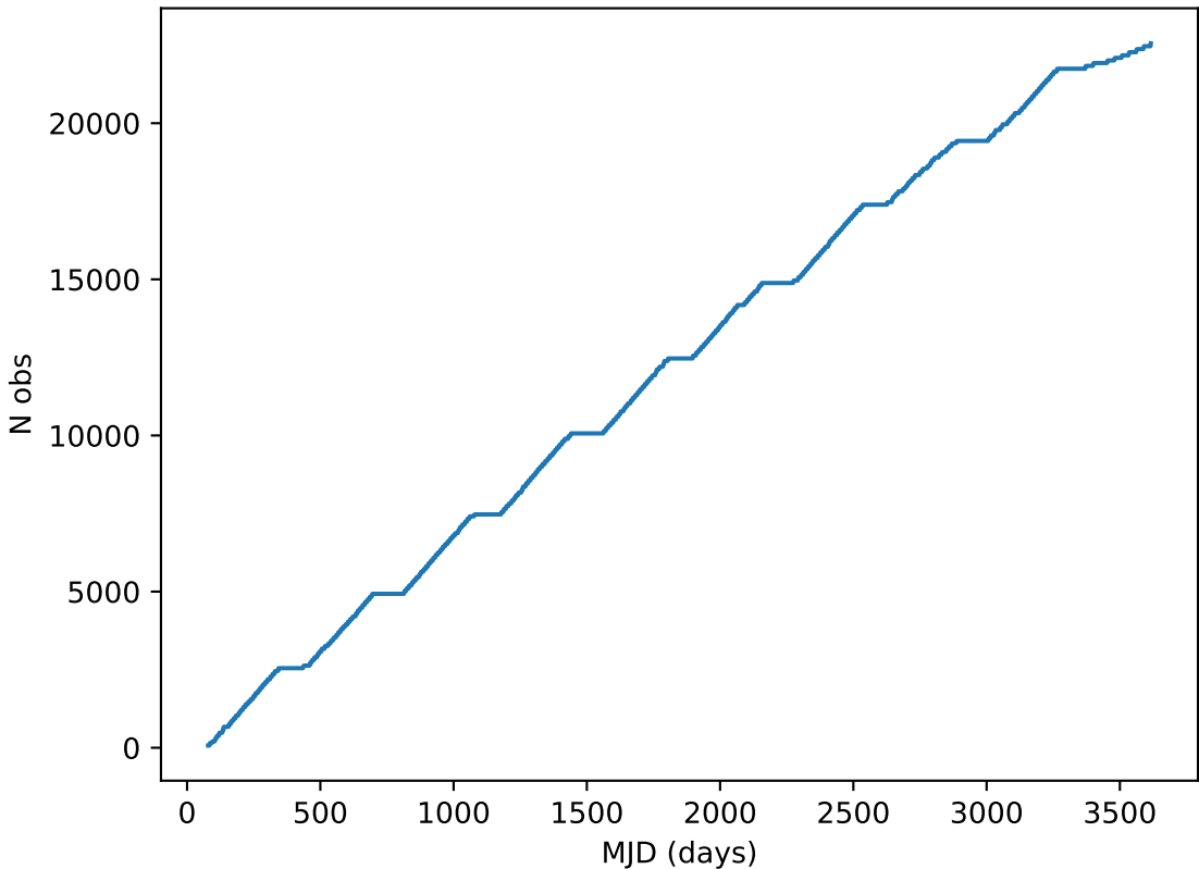
ddf_acor_sf10_lsf15_lsr50_v3.4_10yrs all bands: DD:EDFS Cumulative NVisits
