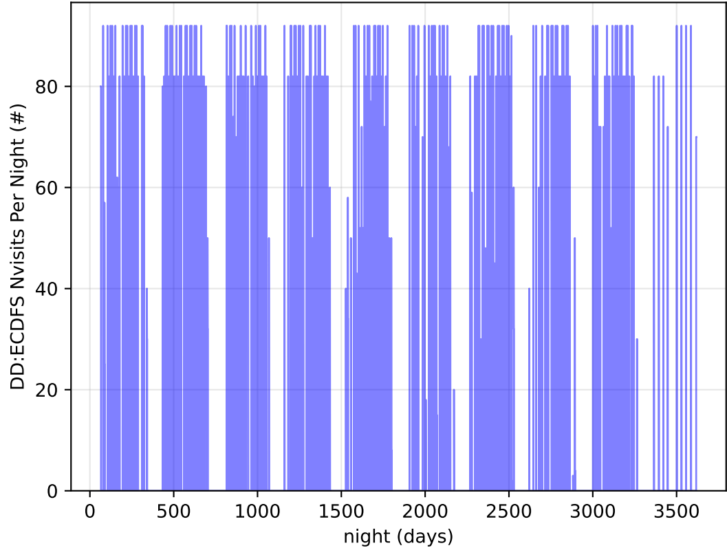
ddf_acor_sf10_ls15_lsr50_v3.4_10yrs all bands: DD:ECDFS Nvisits Per Night
