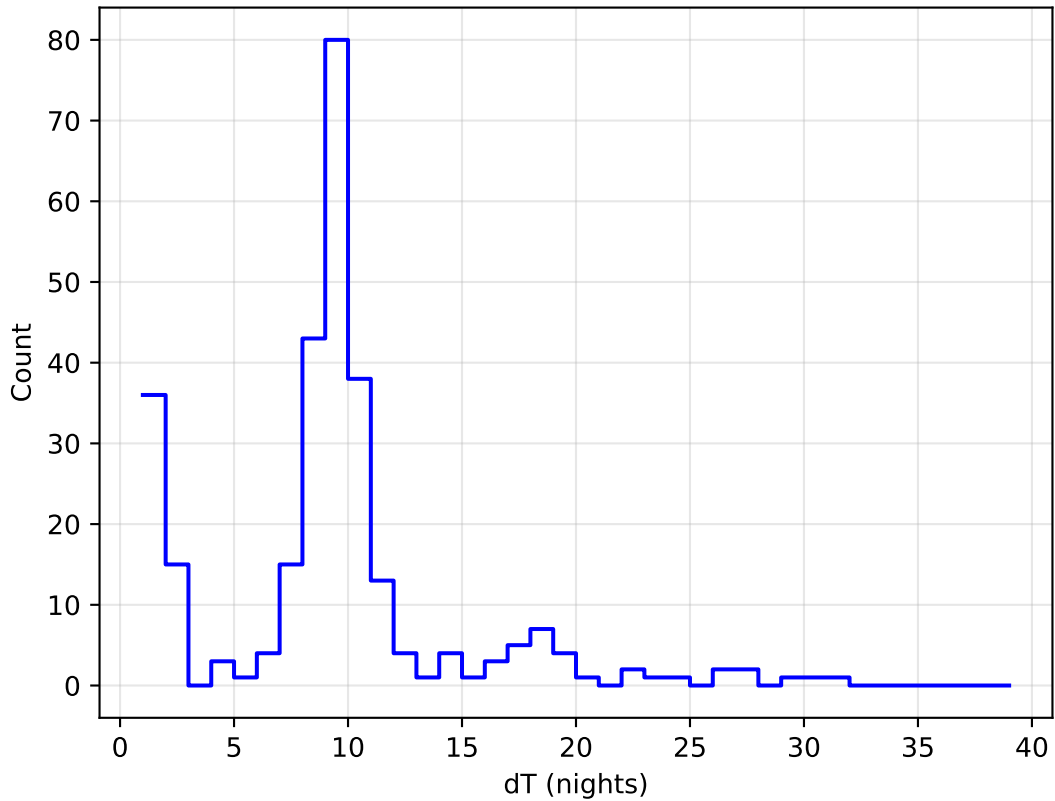
ddf_acor_sf10_lsf15_lsr50_v3.4_10yrs all bands: DD:ECDFS Delta Nights Histogram
