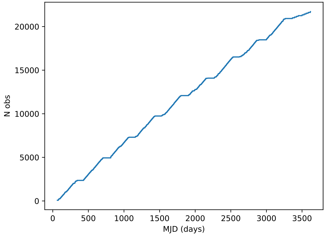
ddf_acor_sf10_lsf15_lsr50_v3.4_10yrs all bands: DD:ECDFS Cumulative NVisits
