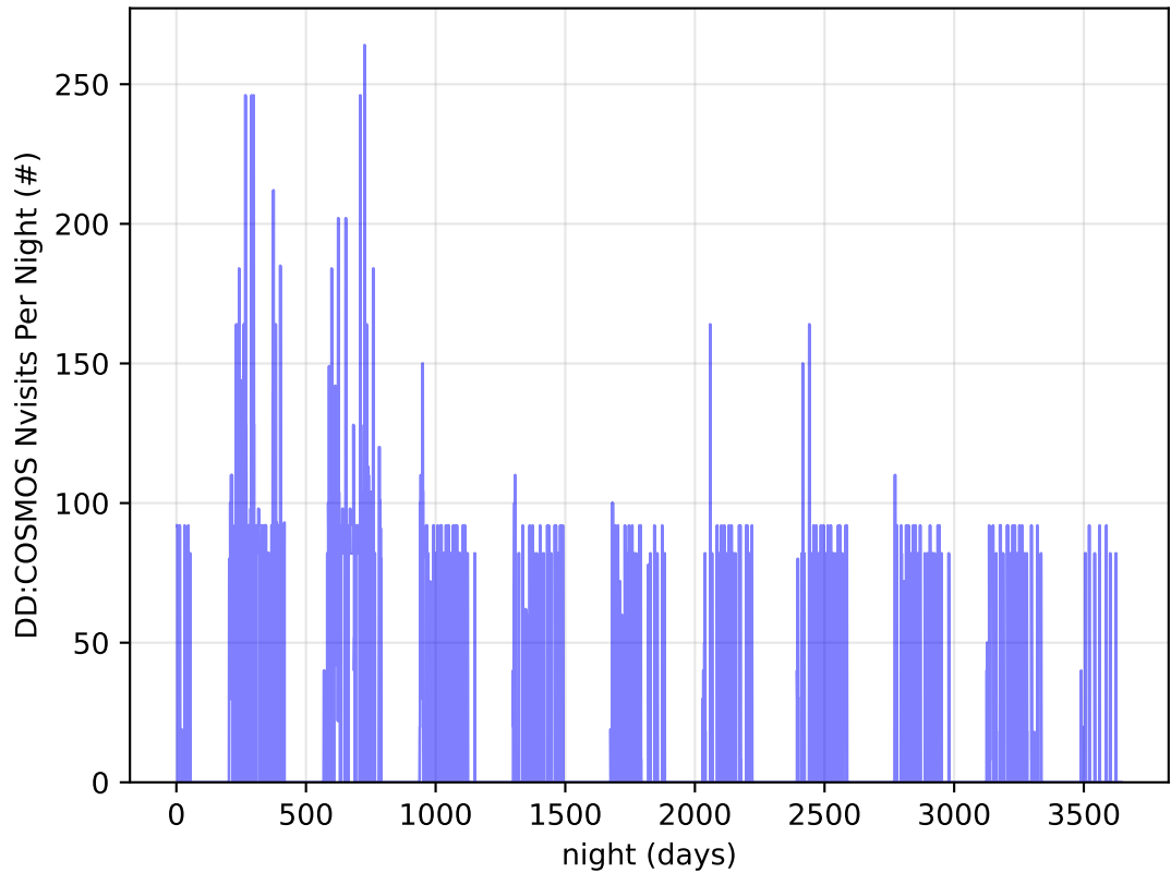
ddf_acor_sf10_lsf15_lsr50_v3.4_10yrs all bands: DD: COSMOS Nvisits Per Night
