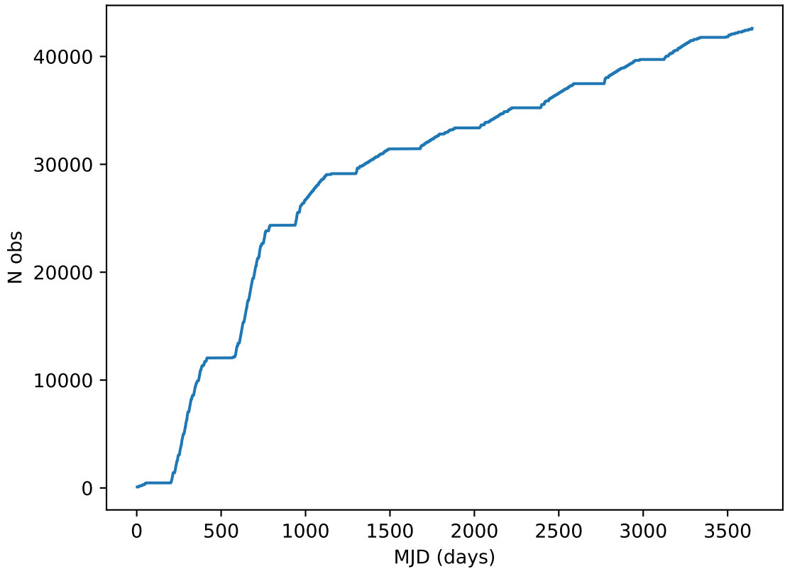
ddf_acor_sf10_lsf15_lsr50_v3.4_10yrs all bands: DD: COSMOS Cumulative NVisits
