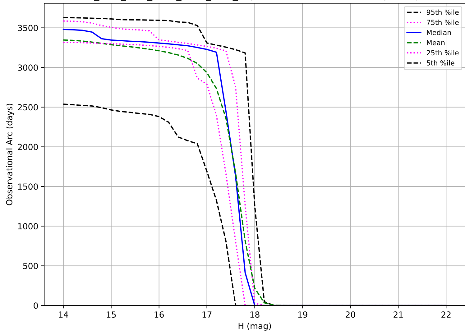
ddf_acor_sf10_lsf15_lsr20_v3.4_10yrs: Observational Arc Length Trojan
