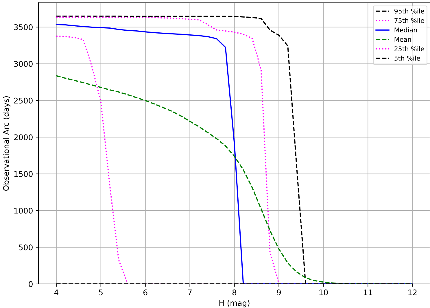
ddf_acor_sf10_lsf15_lsr20_v3.4_10yrs: Observational Arc Length TNO
