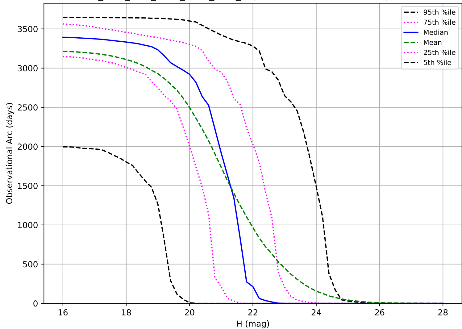
ddf_acor_sf10_lsf15_lsr20_v3.4_10yrs: Observational Arc Length PHA
