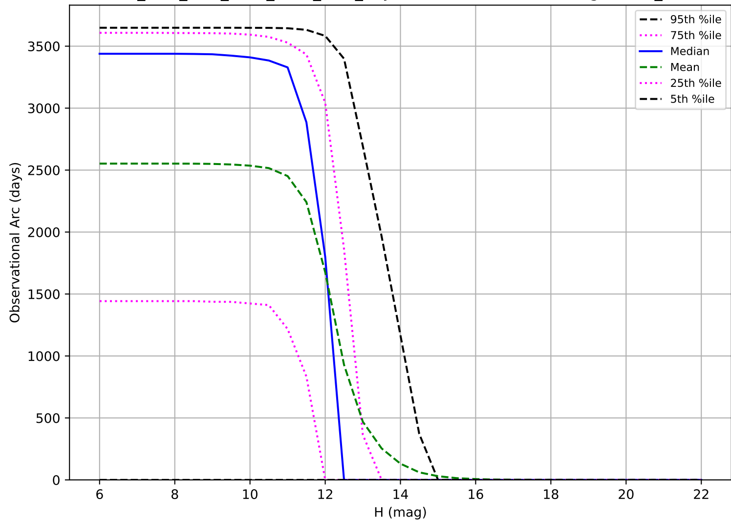
ddf_acor_sf10_lsf15_lsr20_v3.4_10yrs: Observational Arc Length OCC_r20
