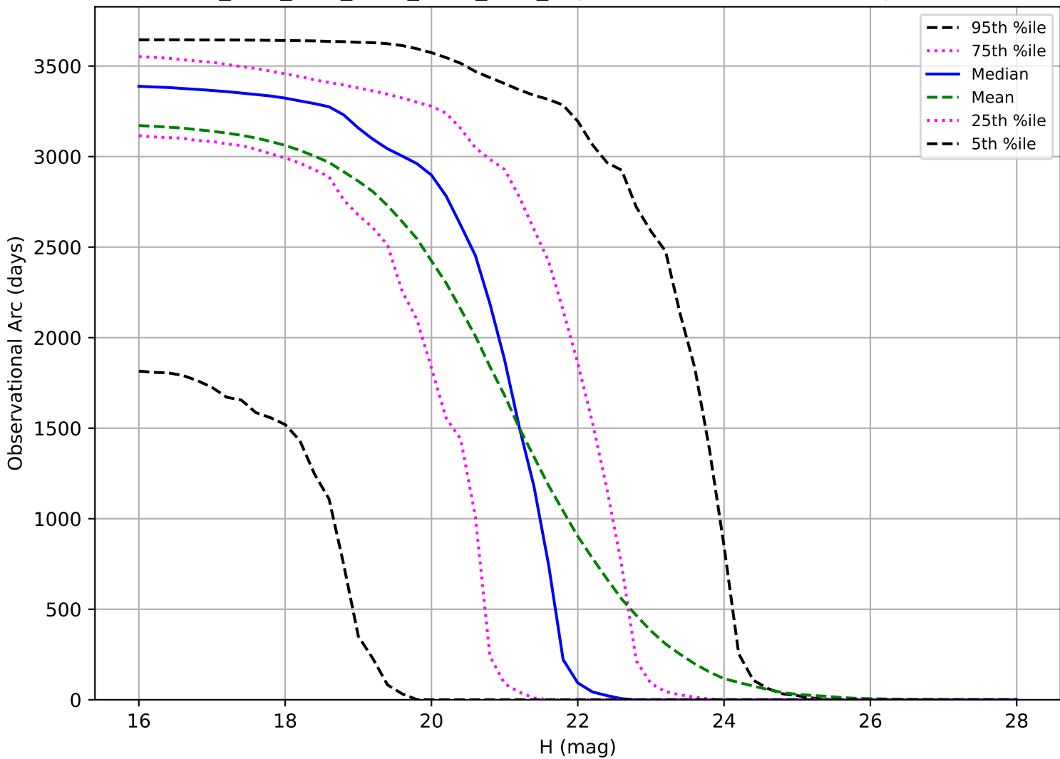
ddf_acor_sf10_lsf15_lsr20_v3.4_10yrs: Observational Arc Length NEO
