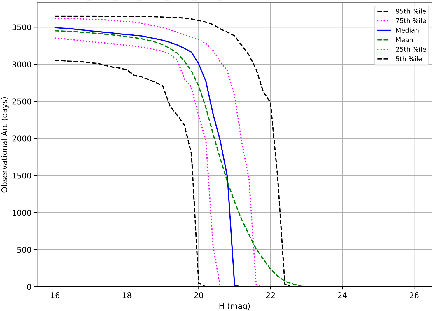
ddf_acor_sf10_lsf15_lsr20_v3.4_10yrs: Observational Arc Length MBA
