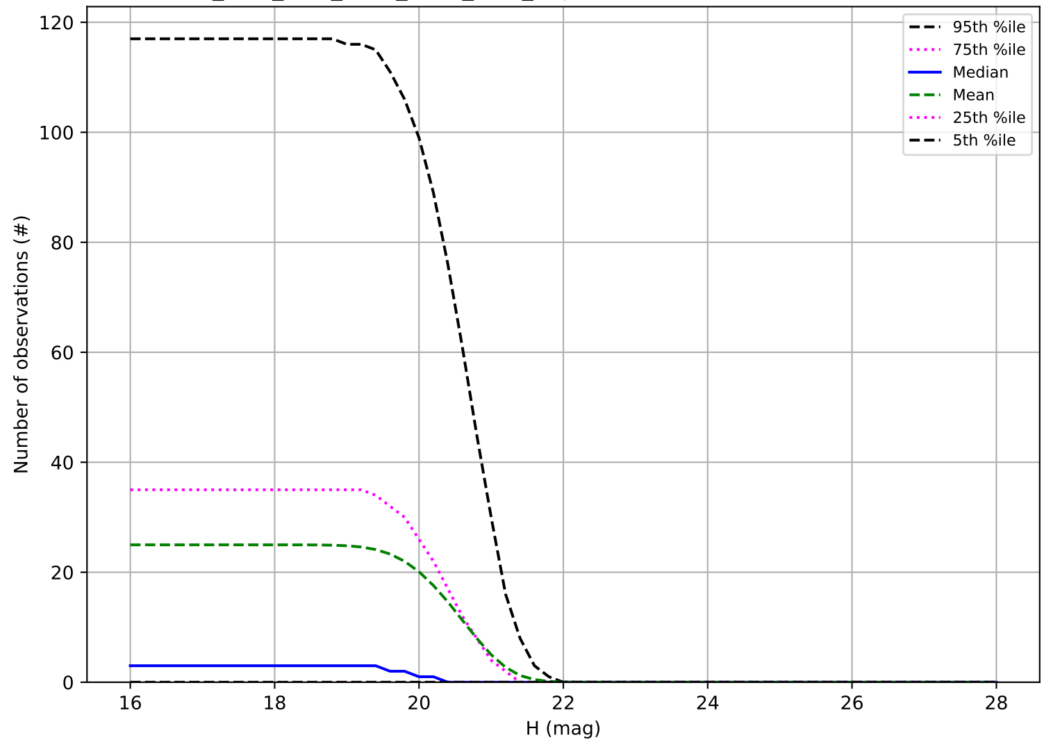
ddf_acor_sf10_lsf15_lsr20_v3.4_10yrs: Number of observations Vatira
