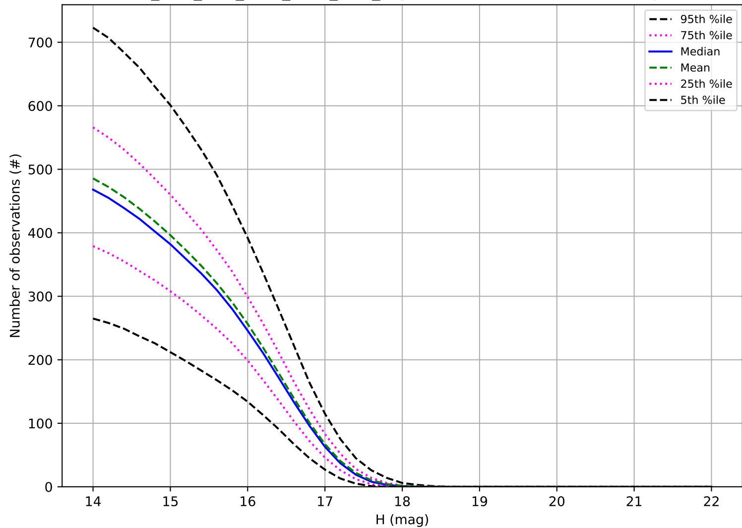
ddf_acor_sf10_lsf15_lsr20_v3.4_10yrs: Number of observations Trojan
