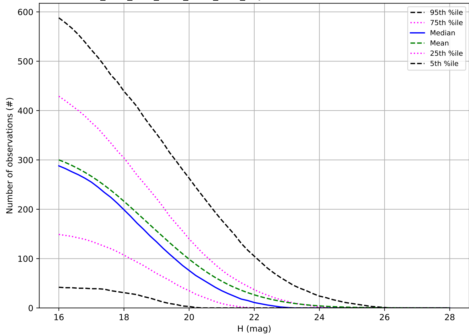
ddf_acor_sf10_lsf15_lsr20_v3.4_10yrs: Number of observations PHA
