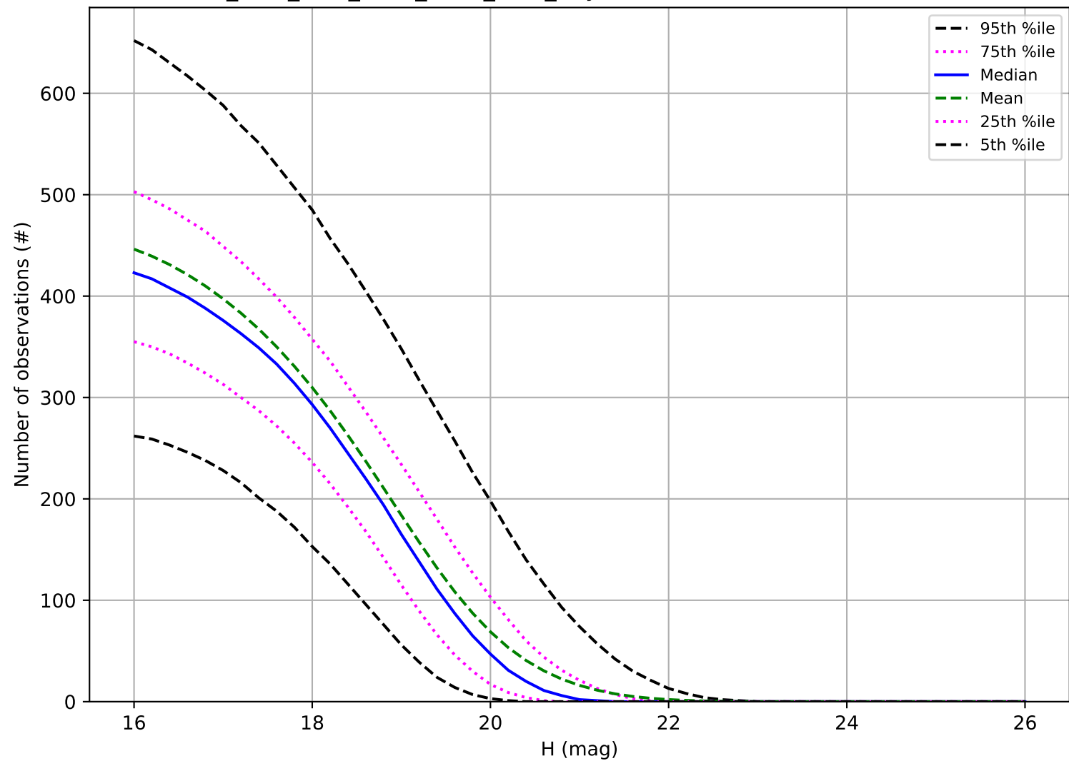
ddf_acor_sf10_lsf15_lsr20_v3.4_10yrs: Number of observations MBA
