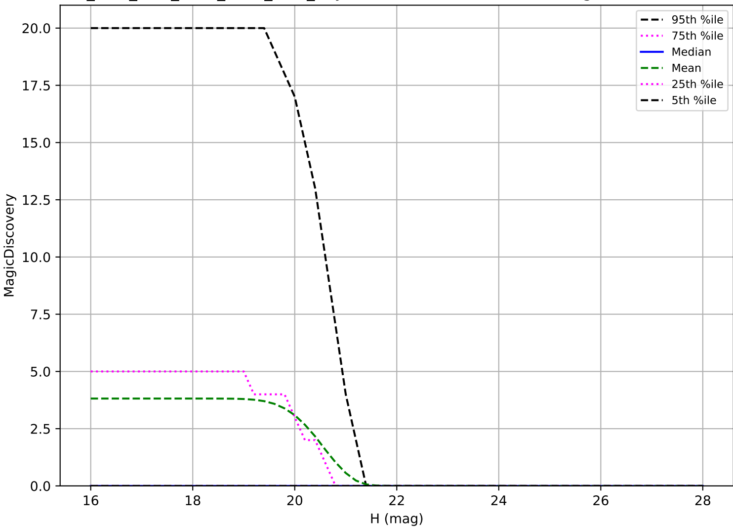
ddf_acor_sf10_lsf15_lsr20_v3.4_10yrs: Vatira 6 detections in 60 nights detection loss
