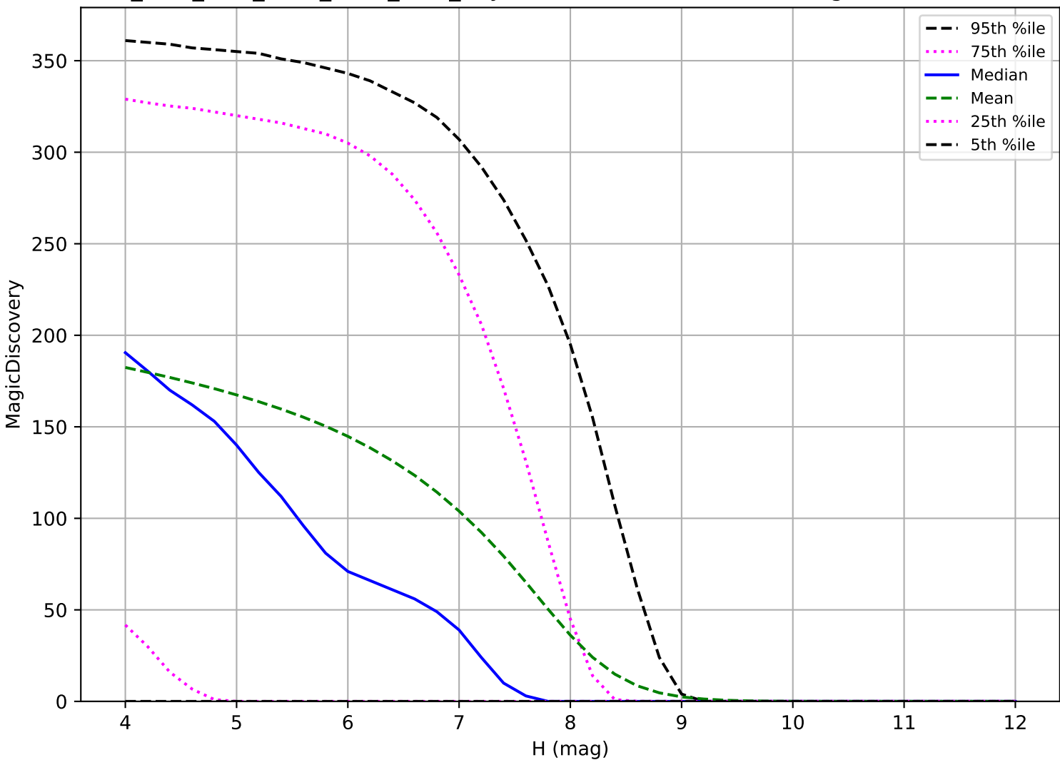
ddf_acor_sf10_lsf15_lsr20_v3.4_10yrs: TNO 6 detections in 60 nights detection loss
